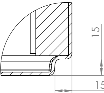
DETAIL C SCALE 1 : 2
